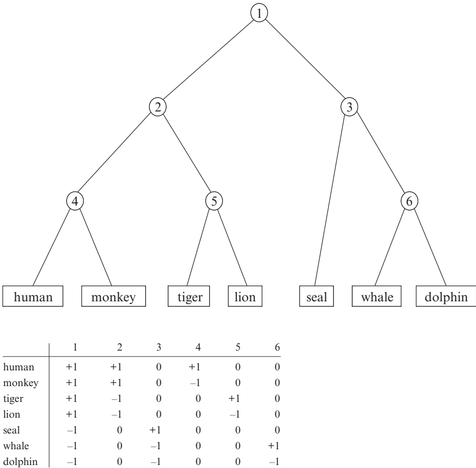
Figure 10.4 Seven classes arranged naturally in a hierarchy, and a corresponding code based on this hierarchy.
